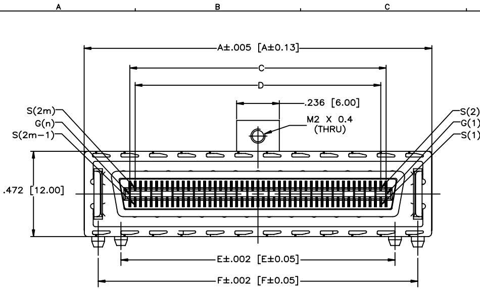
U65-BXX-XX7XXX (LOCK PLATE REMOVED)
