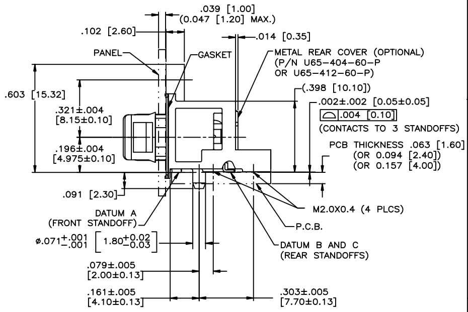
U65-EXX-XX7XXX (SCREW MOUNT)
