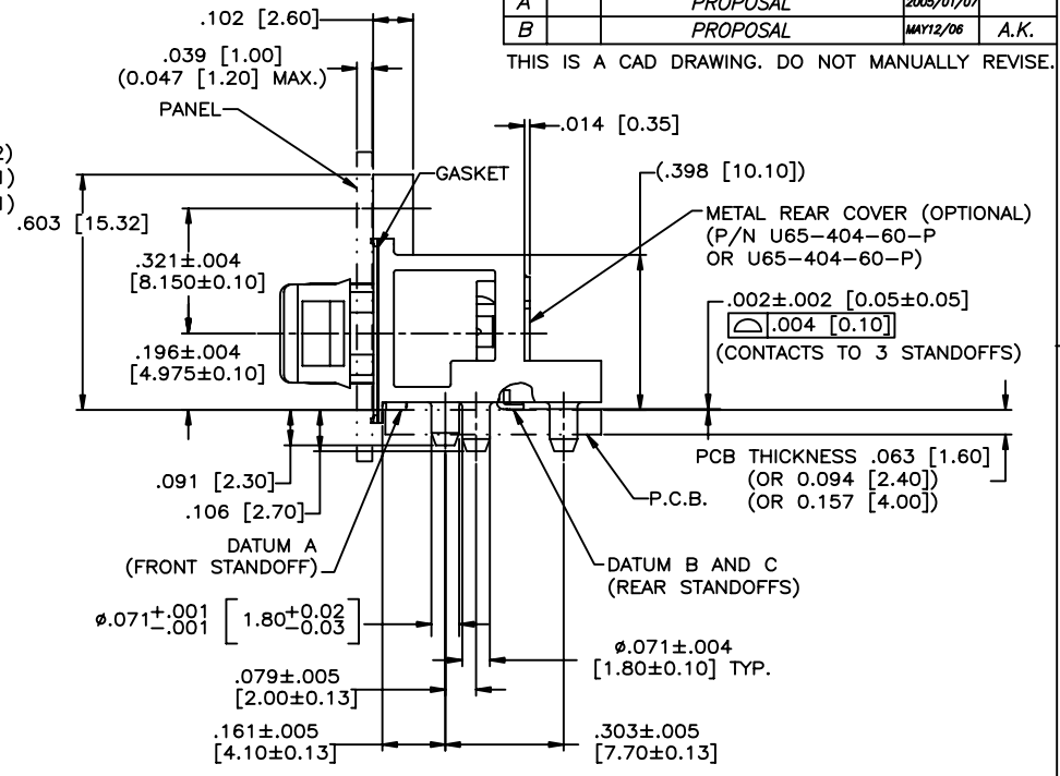
U65-BXX-XX7XXX (SOLDER POST)
