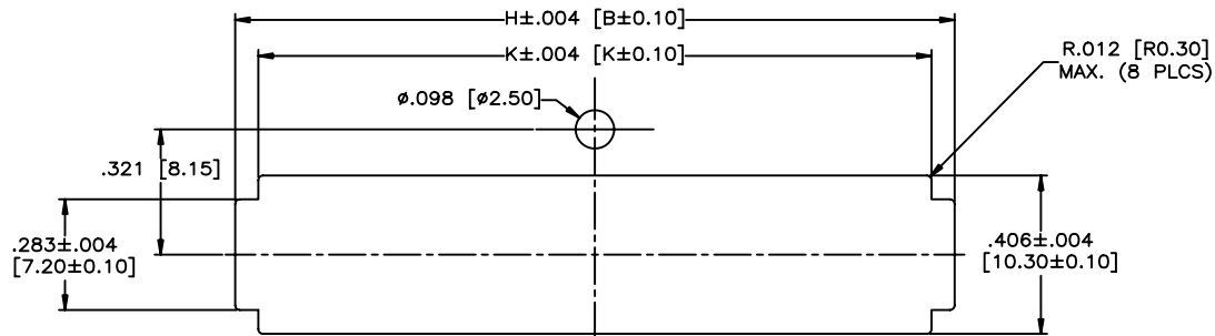
RECOMMENDED PANEL CUTOUT
