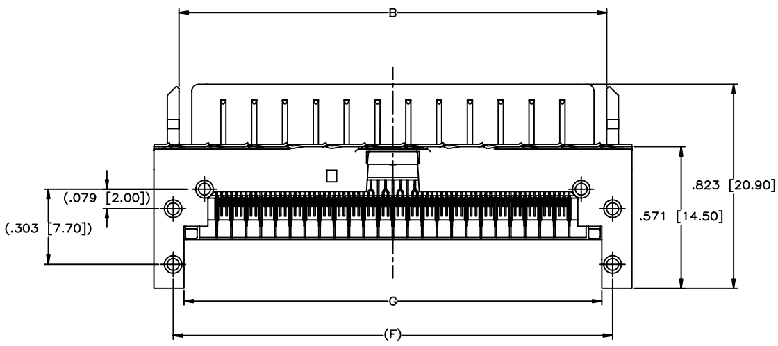
U65-BXX-XX7XXX (LOCK PLATE REMOVED)
